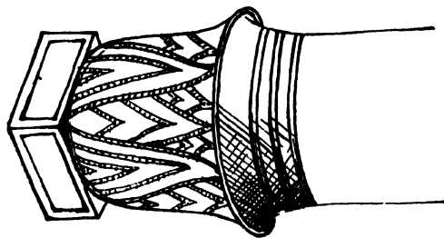
Fig. 2 Capital from the work of Thothmes at Karnak.
